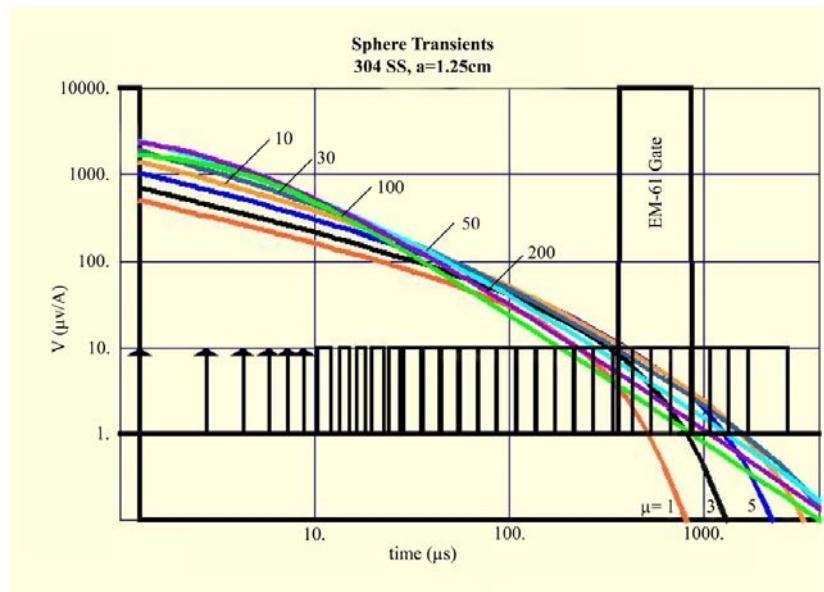
Figure 4: Receiver loop dB/dt transients versus log time. The NanoTEM system records transient values at 31 time windows spaced logarithmically between 0.1 and 2000 \mu sec after the transmitter current pulse. Transient shape can provide diagnostic information about UXO properties. Colored curves show the different transient responses expected from a conductive spherical object with relative permeability values ranging from 1 to 200.
