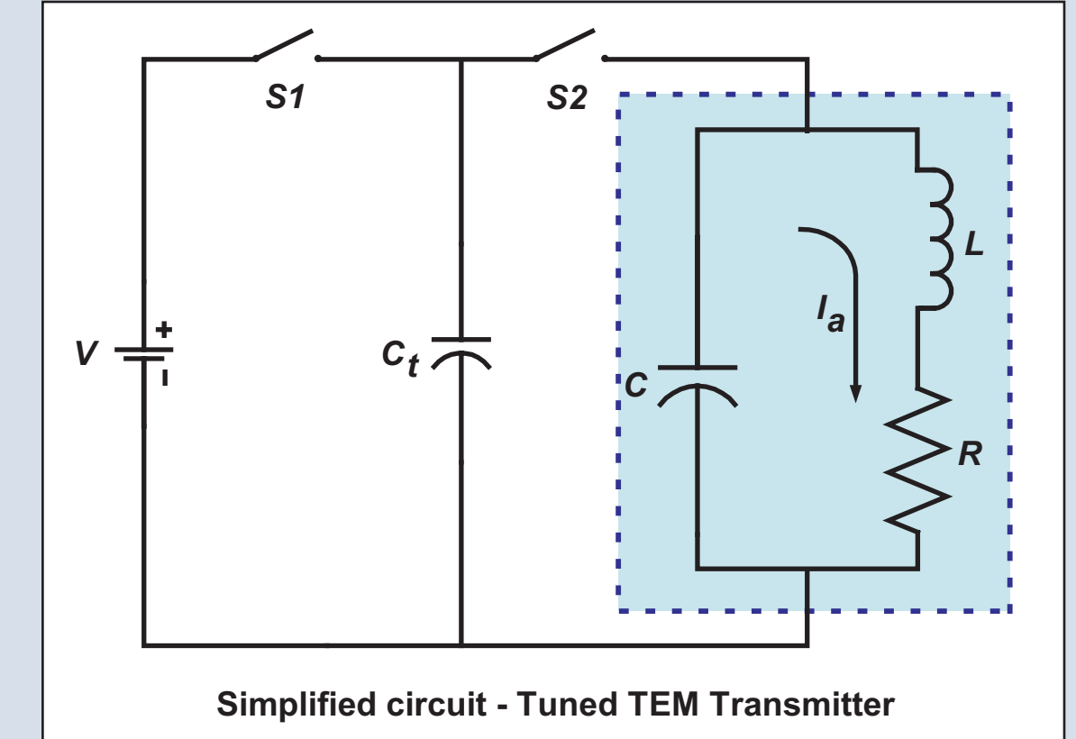
Simplified circuit - Tuned TEM Transmitter
