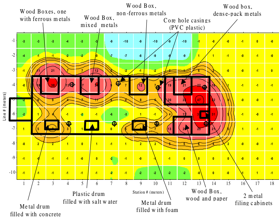
Figure 4: Plan view of in-loop TEM data (Hz component) for several late time windows over the INEL Calibration Cell. Values shown are the average of windows 21 through 26 in microvolts/am pere, contoured logarithmically.
