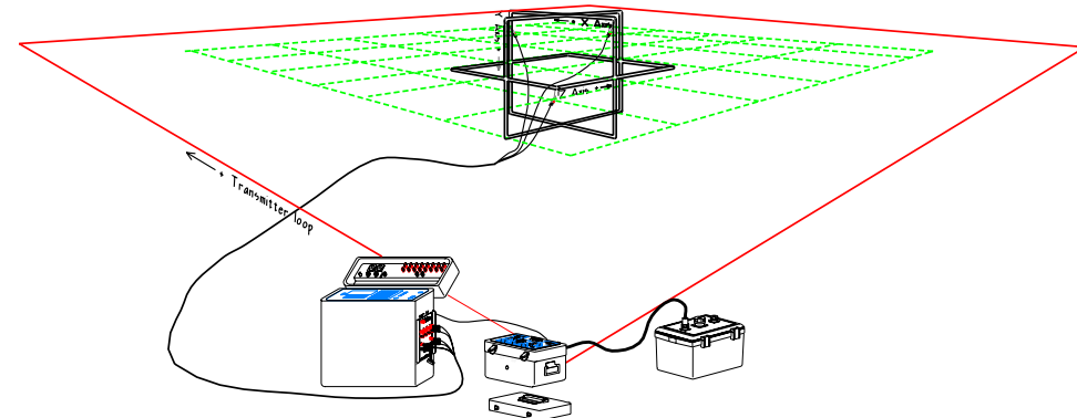
Setup Diagram of NanoTEM System
